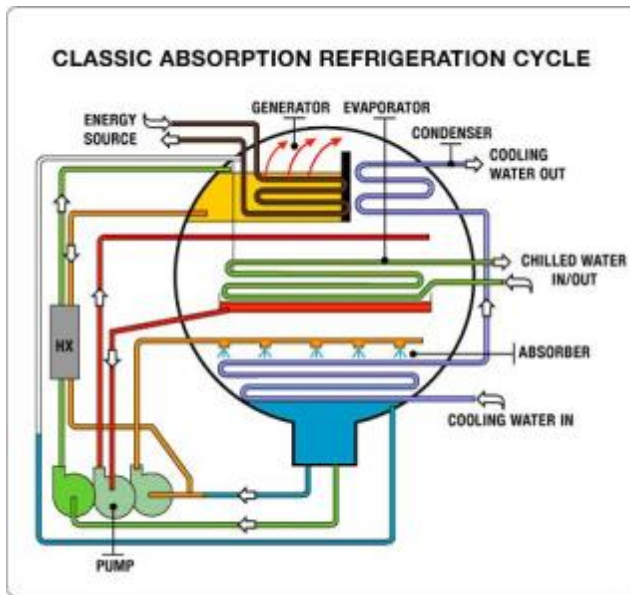
Fig. 4: Schematic of an absorption chiller [2]
