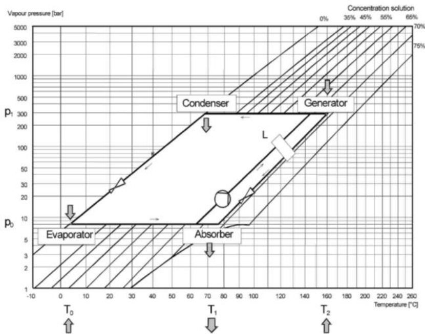
Fig. 5: Cooling cycle of an absorption process. Vapour pressure as a function of vapour temperature.
