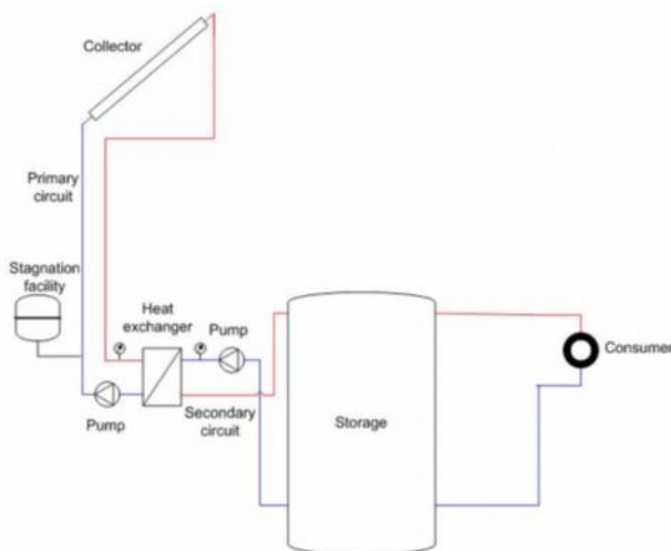
Fig. 1: Basic scheme of a solar thermal plant
