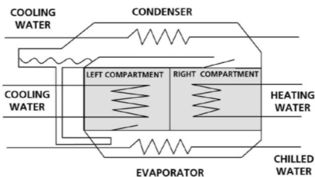
Fig. 6: Schematic of the internal chambers of an adsorption chiller [Error! Bookmark not defined.]
