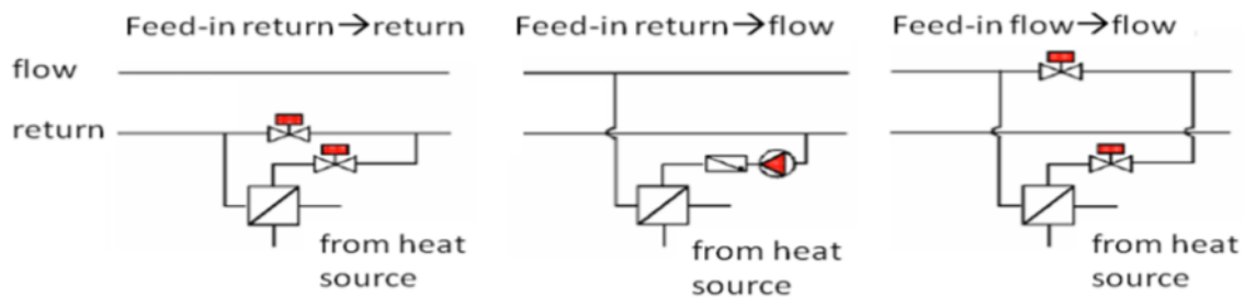
Fig. 2: Hydraulic integration of solar thermal feed-in (source: Wolfgang Streicher)
