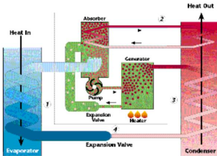
Fig. 16: Absorption heat pump
