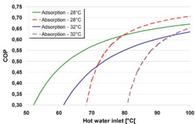
Fig. 7: COP of adsorption and absorption chiller as a function of heating water temperature (chilled water 9°C, cooling water 28 and 32 °C); [Error! Bookmark not defined.]
