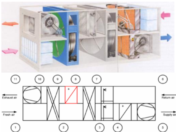
Fig. 8: Schematic of an Desiccant cooling system Cooling cycle
